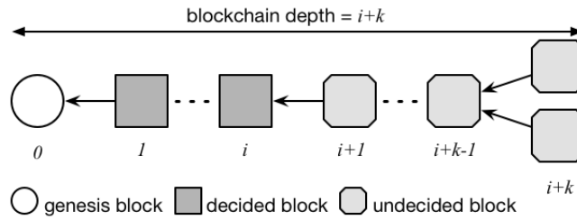
Figure 2: The blockchain structure starts with a genesis block at index 0 and links successive blocks in reverse order of their index; a new block is decided at index i > 0 when the blockchain depth reaches i + k (note that a blockchain of depth 0 is the genesis block)
