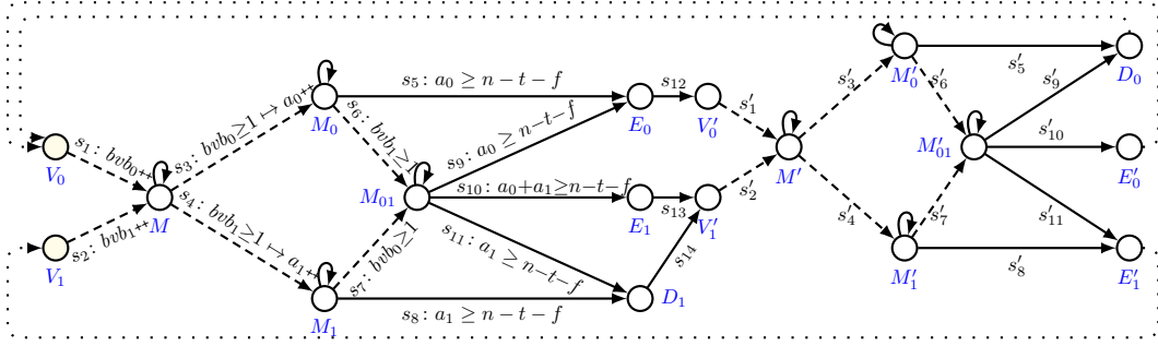
■ Figure 4 The simplified threshold automaton of the Byzantine consensus of Algorithm 1 obtained after model checking the bv-broadcast . Rules s'_j , 1 \leq j \leq 11 , are obtained from s_j by replacing each variable c \in \{a_0, a_1, bvb_0, bvb_1\} with its corresponding one c' .
